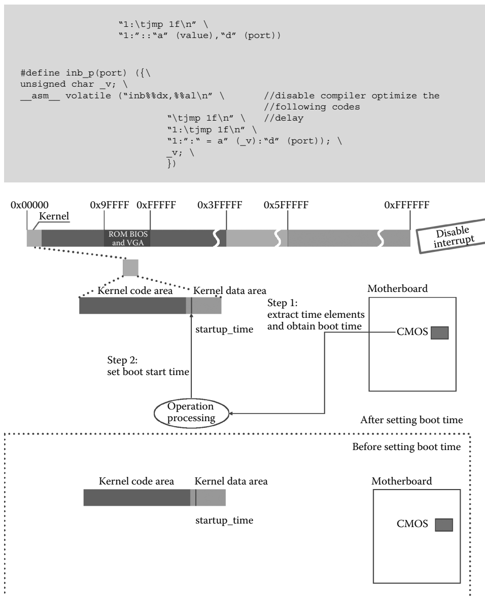
Figure 2.15 Boot time setting.
