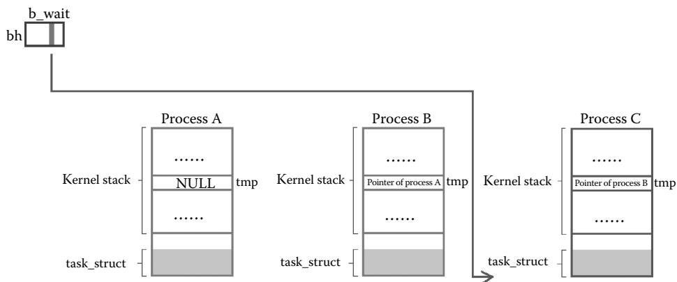
Figure 7.22 Process C was set to TASK_UNINTERRUPTIBLE and added to the process wait queue.
