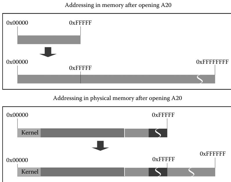
Figure 1.19 Open A20.
