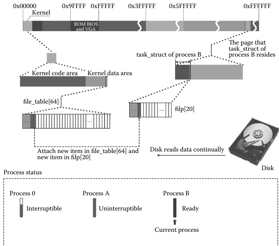
Figure 7.15 System build relationships between process B and the kernel file management table.
