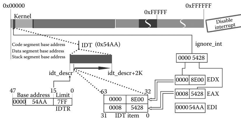
Figure 1.28 Set IDT.
