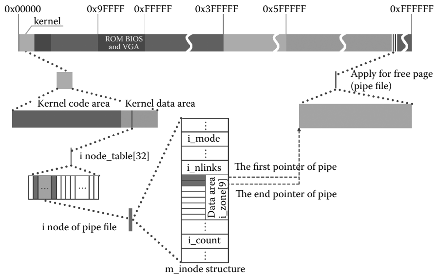
Figure 8.4 Create i node for pipe file.
