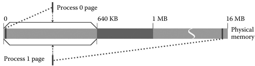
Figure 3.9 Process 0 and process 1 share the same page.
