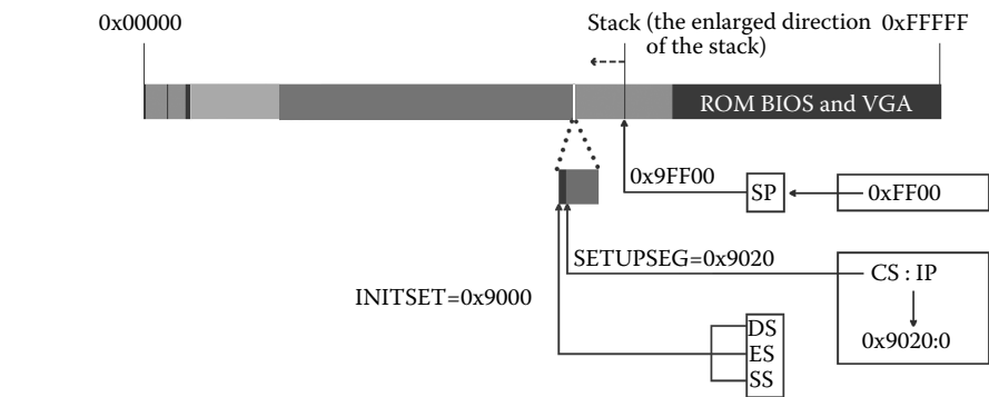
Figure 1.14 Setup begins to execute.
