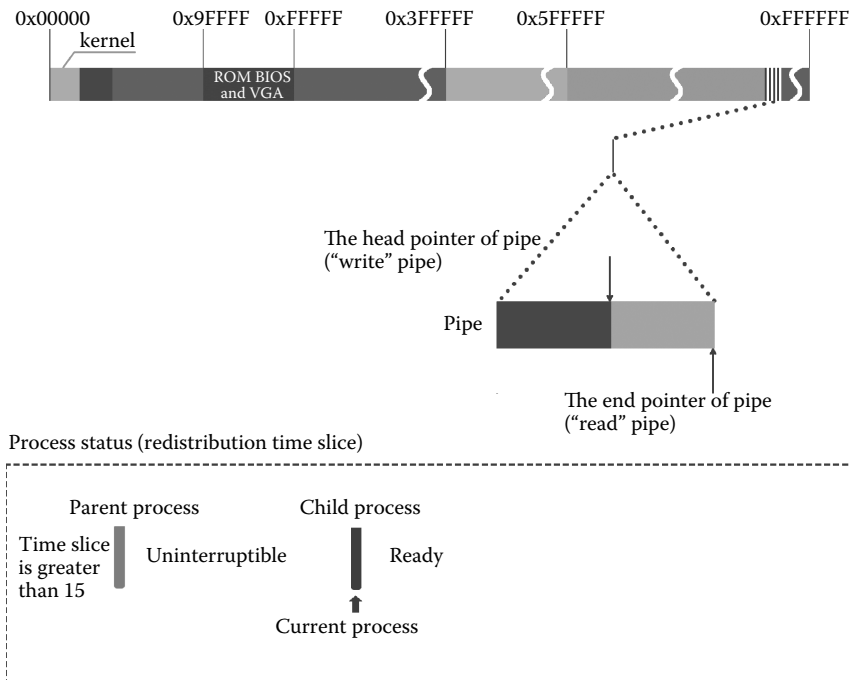
Figure 8.17 Read pipe process continues to read data from the pipe.
