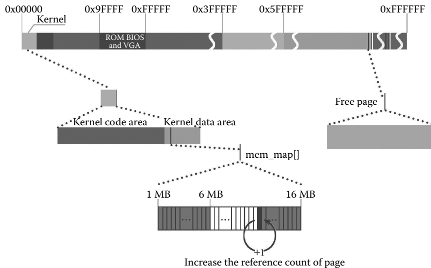
Figure 6.14 Allocate a memory page for strl.
