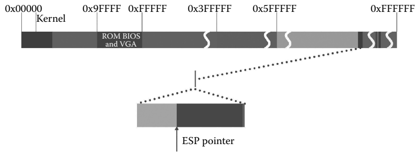
Figure 6.17 The first time strl pushing stack.
