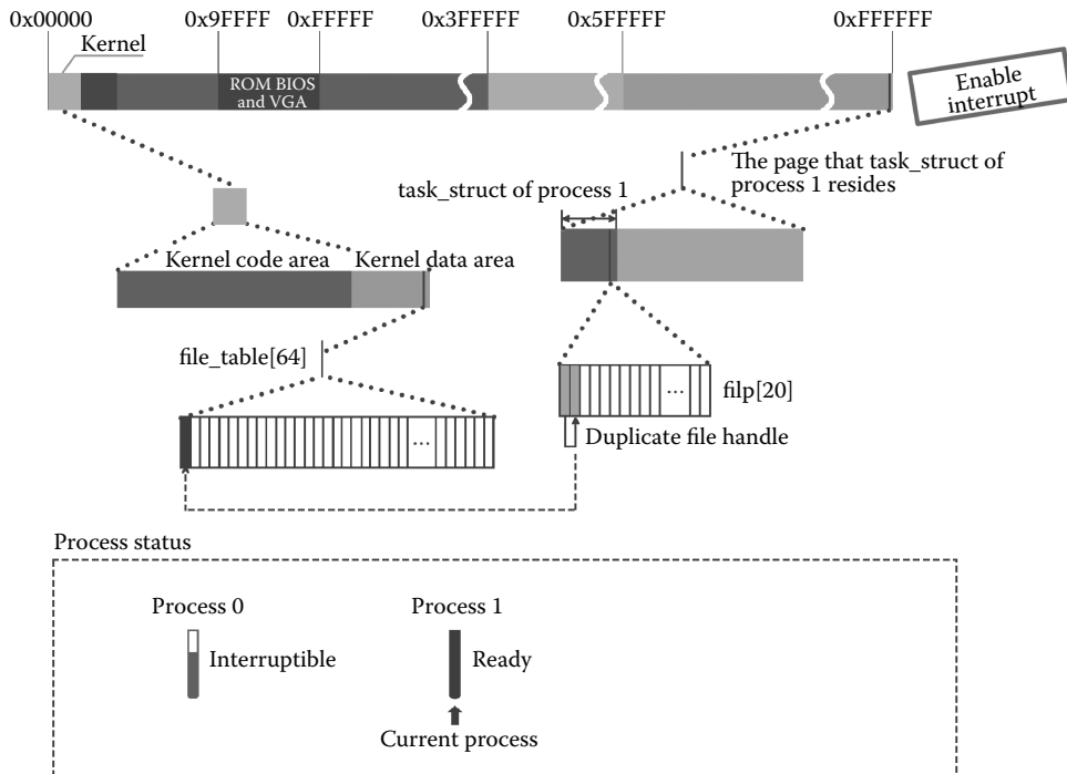
Figure 4.9 Duplicate the filp[fd] and open std output device.
