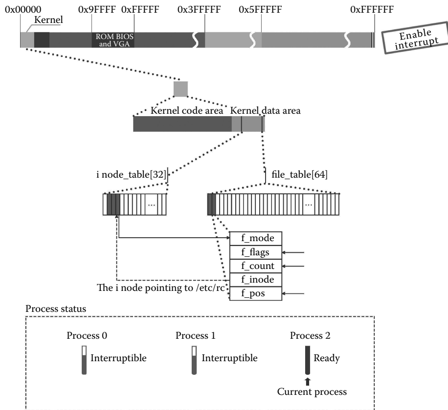
Figure 4.19 Open/etc/rc.
