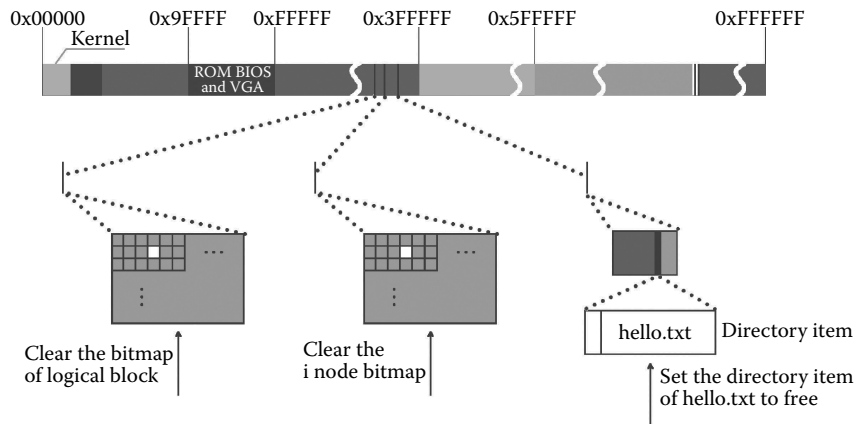
Figure 5.14 Delete the file hello.txt.
