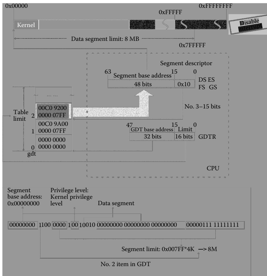
Figure 1.26 Set DS, ES, FS, and GS.
