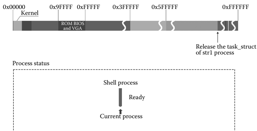
Figure 6.22 Str1 process exit, switch to shell process.
