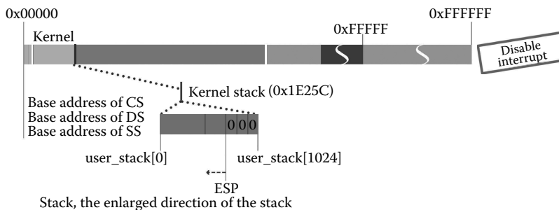
Figure 1.34 Push evnp, argv, and argc.
