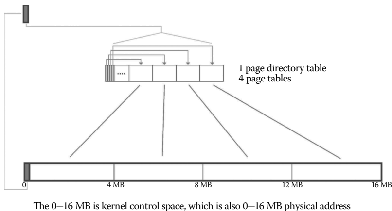
Figure 6.3 Kernel paging.
