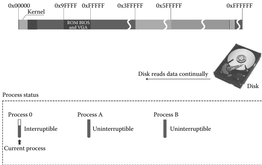
Figure 7.18 Process B was set to TASK_UNINTERRUPTIBLE.
