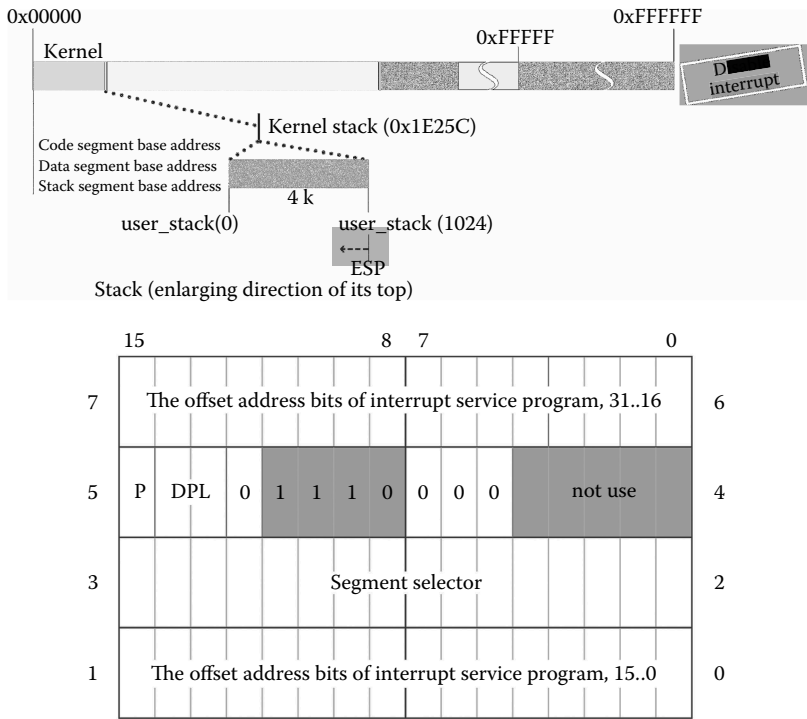
Figure 1.27 Set stack.
