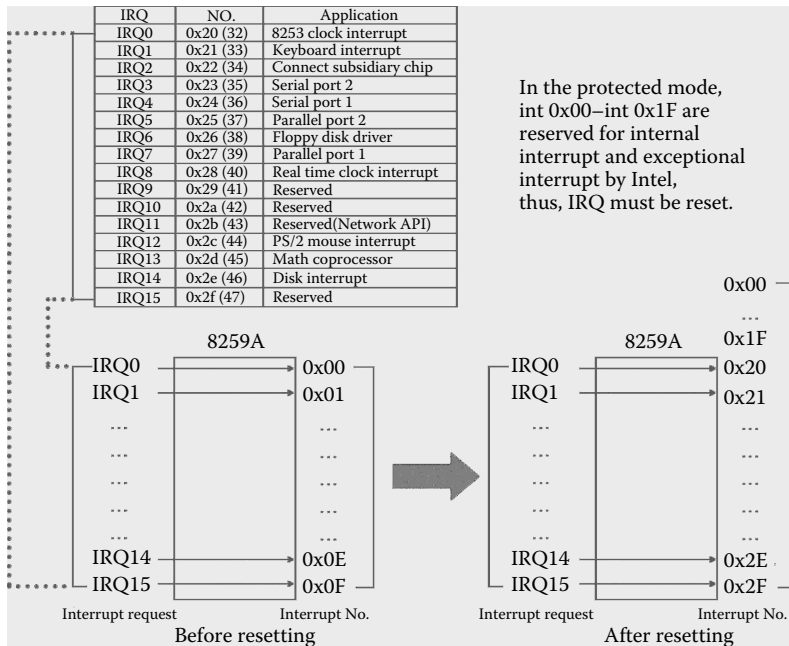
Figure 1.20 Resetting 8259A.
