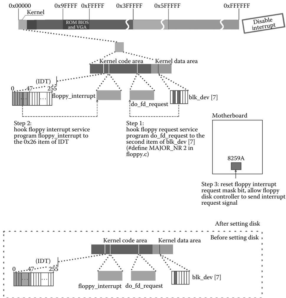
Figure 2.27 Initialize the floppy disk.
