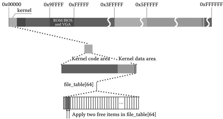
Figure 8.2 Two free entries that are applied for in file_table[64] for creating the pipe file.
