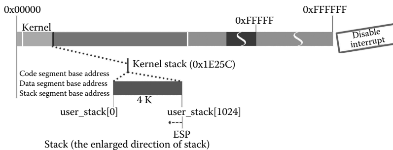
Figure 1.31 Set the kernel stack.
